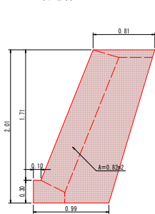
目地材C S=1:25
